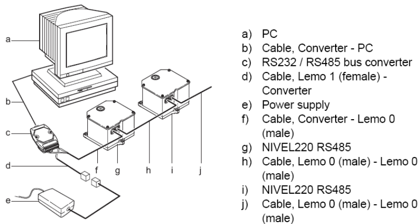
Figure 4: Tiltmeter to PC Connection
