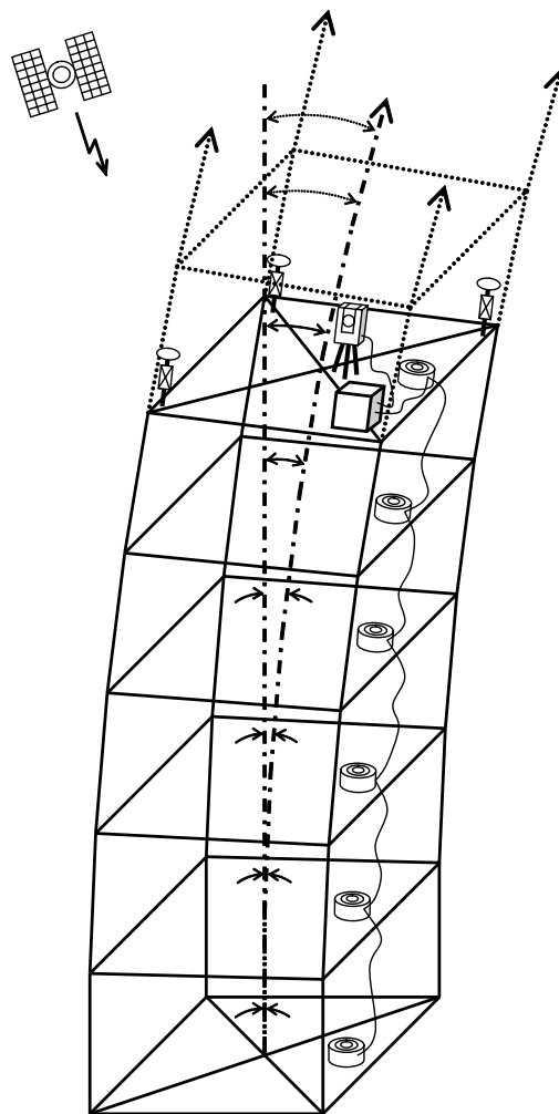
Figure 5: Data Fusion System
